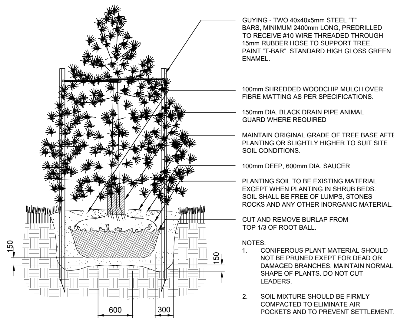
CONIFEROUS TREE PLANTING DETAIL
